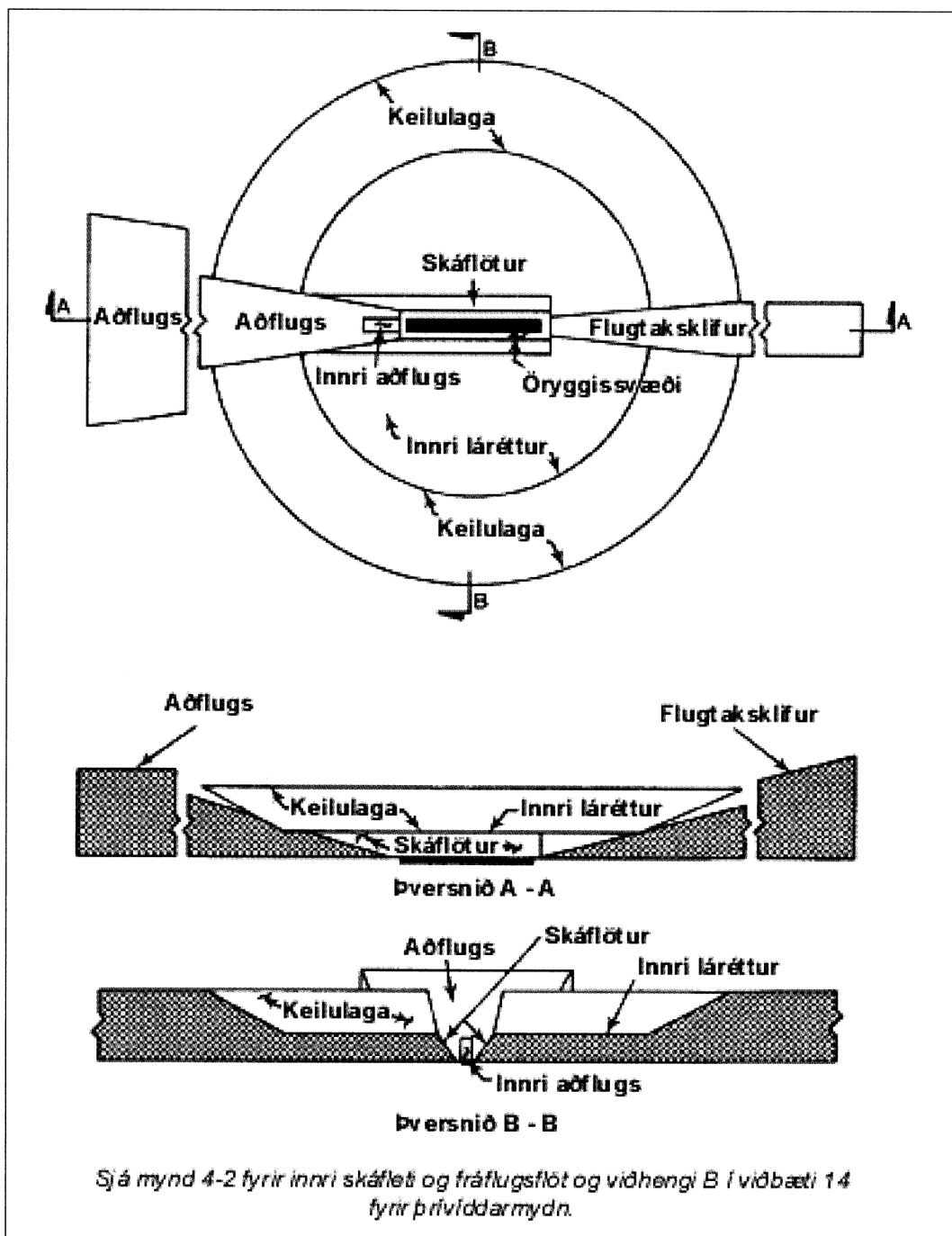
Mynd 4-1. Hindranaflétir (Obstacle limitation surfaces).
