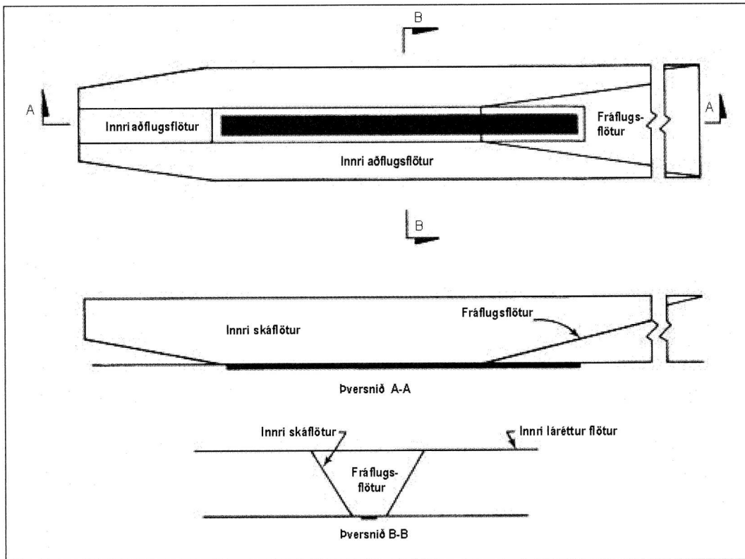
Mynd 4-2. Innri aðflugshindranaflötur, innri skáhindranaflötur og fráflugshindranaflötur (Inner approach, inner transitional and balked landing obstacle limitation surfaces).
