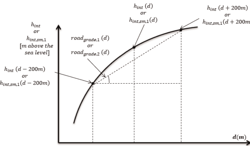
Illustration of the procedure to smooth the interpolated altitude signals
