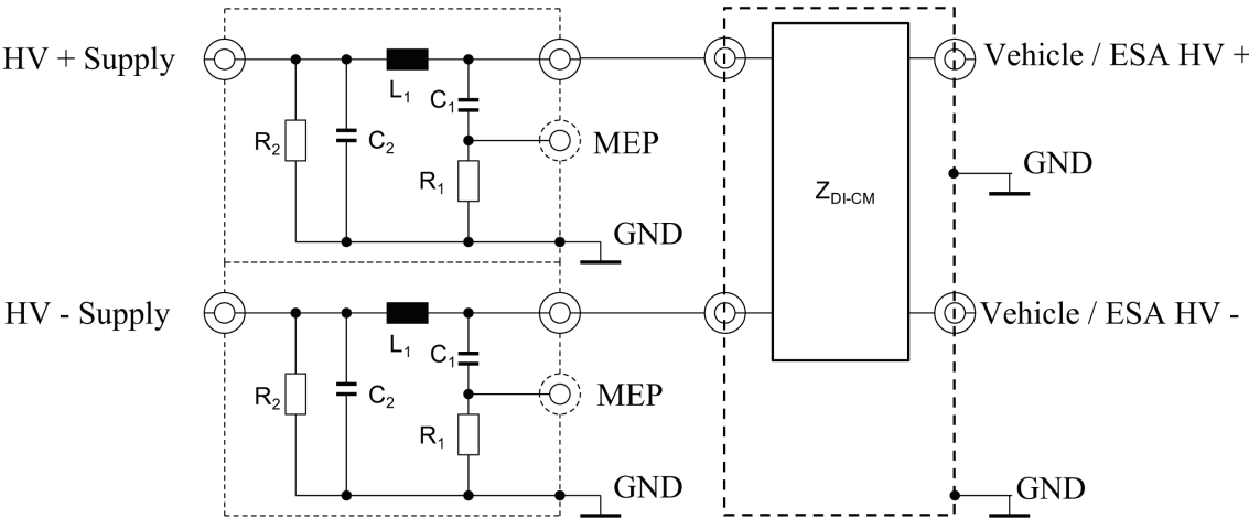
Impedance matching network attached between HV ANs and ESA
