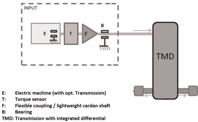
Test setup A for transmission with integrated differential
