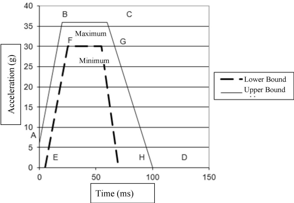
Acceleration Pulse Corridor
