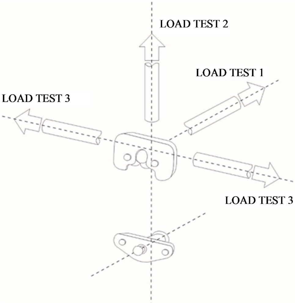
Figure 3-4 Door static load test directions
