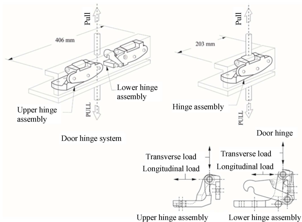
Figure 5-2 Static load test directions for doors that open in the vertical direction
