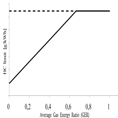
Diagram showing HC emission limit as function of average GER
