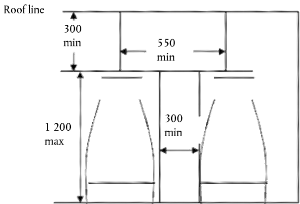
Figure 4 Determination of unobstructed access to door (dimensions in mm) (See Annex 3, paragraph 7.7.1.9.2)
