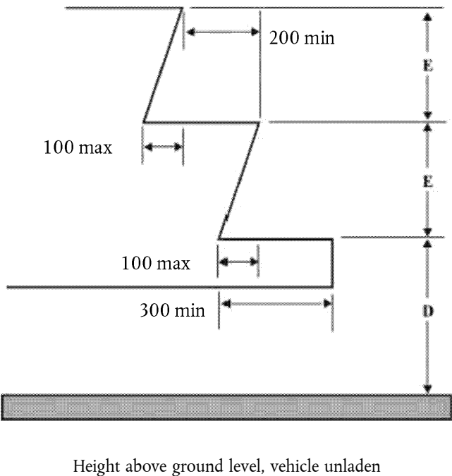
Figure 8 Steps for passengers (dimensions in mm) (See Annex 3, paragraph 7.7.7)
