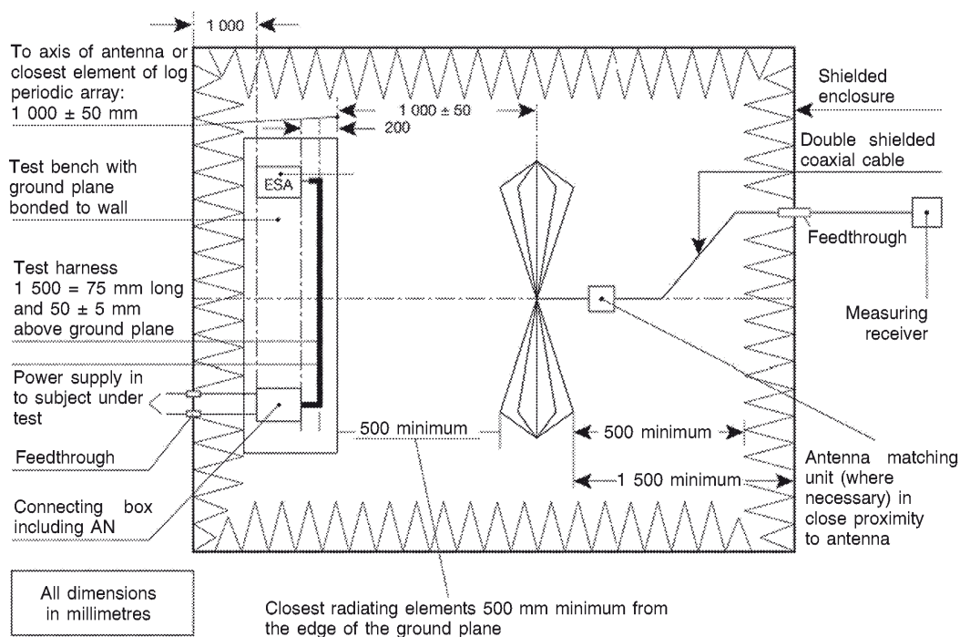
Test layout (general plan view)
