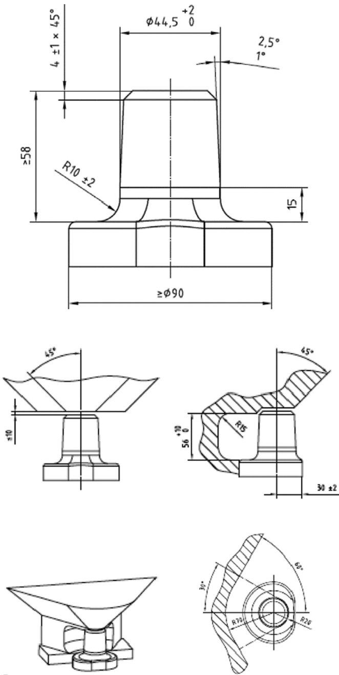
Figure 5 Pin type coupling (corresponding to ISO 6489-4:2004)
