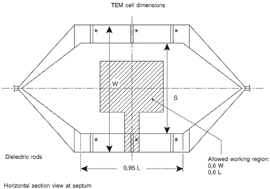
Figure 7 Design of rectangular TEM cell — typical TEM cell dimensions
