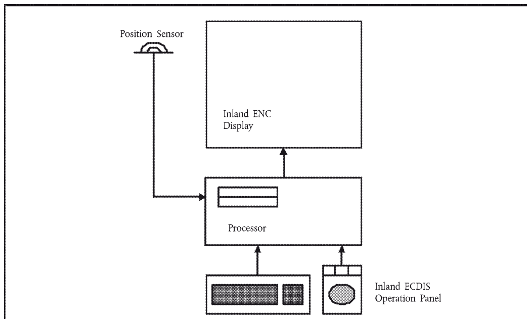
Inland ECDIS equipment, self-sufficient system without connection to radar
