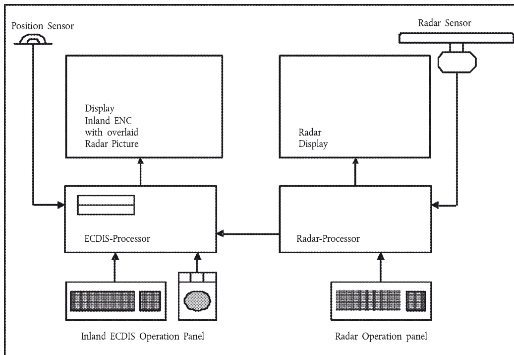
Inland ECDIS equipment, parallel installation with connection to radar
