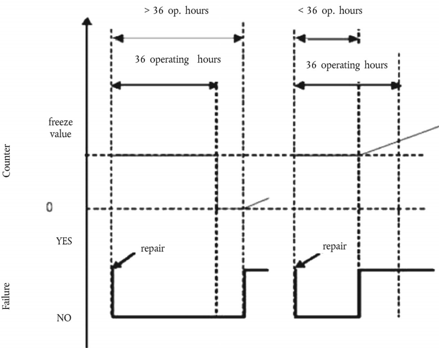
Reactivation and resetting to zero of a counter after a period when its value has been frozen
