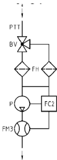
Scheme of particulate sampling system
