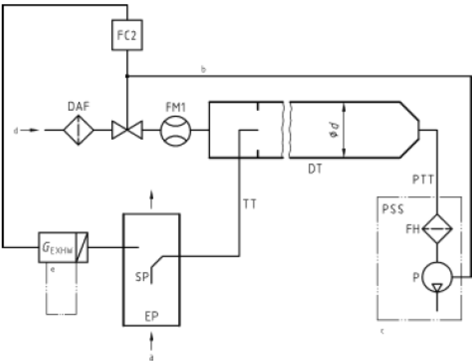
Scheme of partial flow dilution system (total sampling type)
