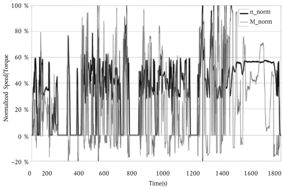
Figure 3 WHTC test cycle
