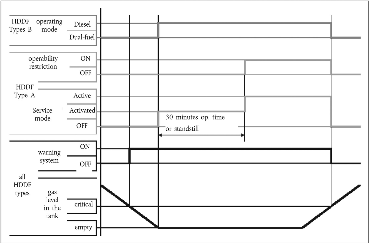
Illustration of the events occurring in case of an empty gas tank (Types A and B HDDF)
