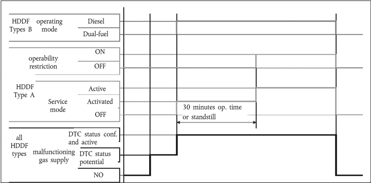
Illustration of the events occurring in case of a malfunctioning gas supply system (Types A and B HDDF)
