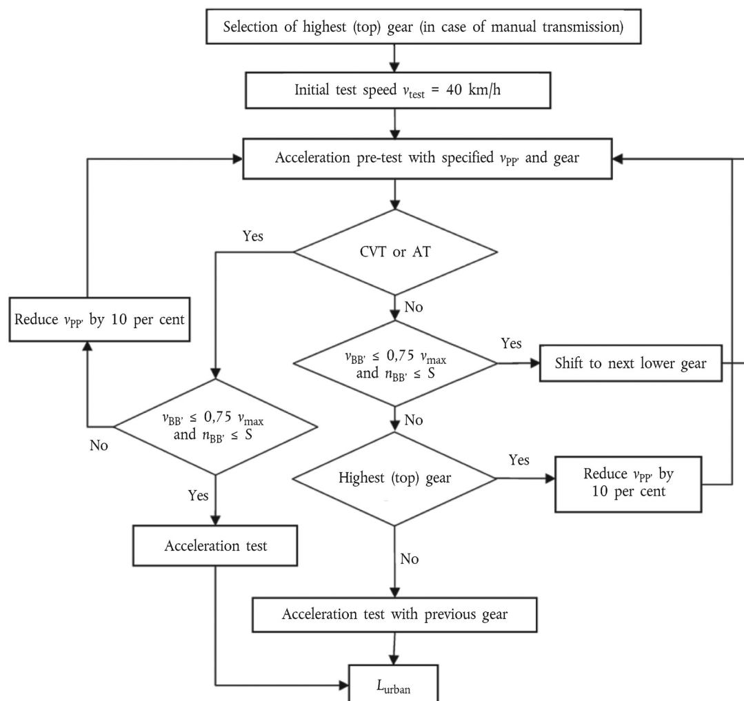
Flowchart of the test procedure for the test of the vehicle in motion for vehicles of category L 3 with PMR ≤ 25
