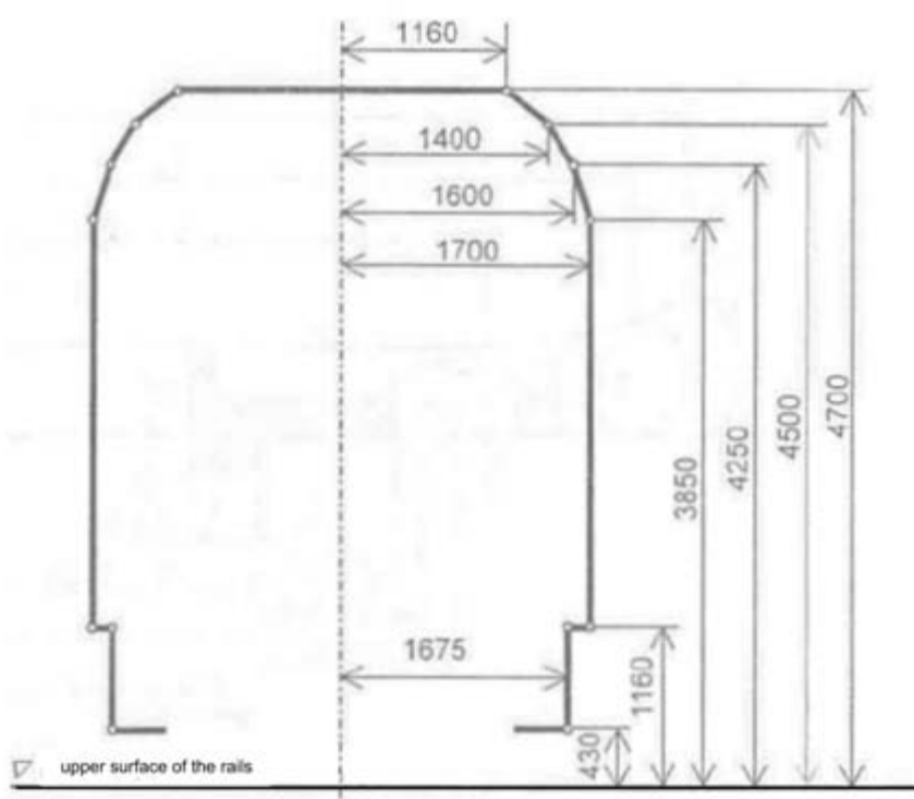
Kinematic gauge WM-1
