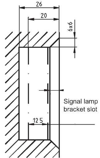
Cross section A-A
