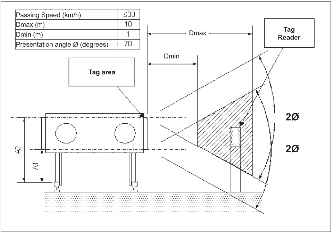
Fig. F2 Installation constraints for tag readers
