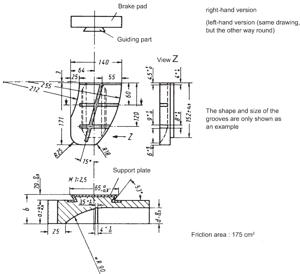
BRAKE PAD (175 cm 2 )
