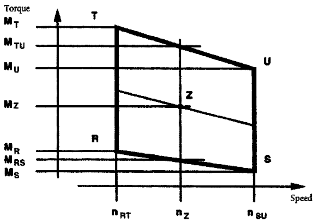
Interpolation of \text{NO}_x Control Point
