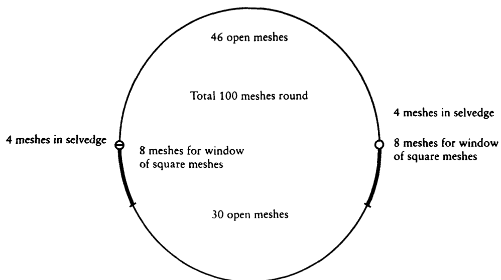
Codend cross section
