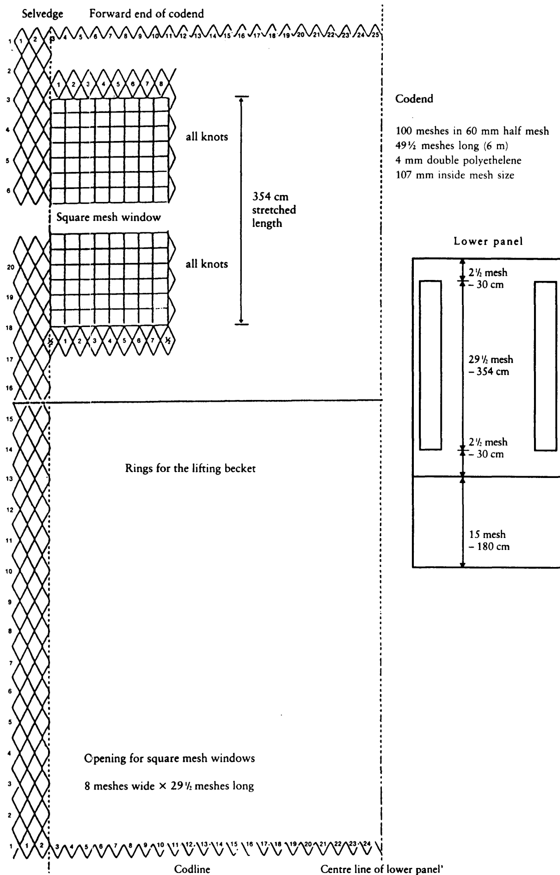
Figure 3: Inserting the window in the codend
